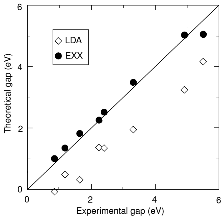
Figure 7: Gaps of common semiconductors calculated using LDA and EXX. Note that Ge is a metal in the best LDA calculations, but the gaps are in much better agreement with experiment using EXX. From Staedele, et al.)
