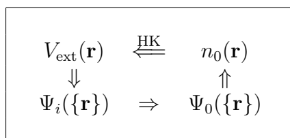
Figure 1: Fig. 6.1 of Text. Schematic representation of Hohenberg–Kohn theorem. The smaller arrows denote the usual solution of the Schrödinger equation where the potential V_{\text{ext}}(\mathbf{r}) determines all states of the system \Psi_i(\{\mathbf{r}\}) , including the ground state \Psi_0(\{\mathbf{r}\}) and ground state density n_0(\mathbf{r}) . The long arrow labeled “HK” denotes the Hohenberg–Kohn theorem, which completes the circle.
